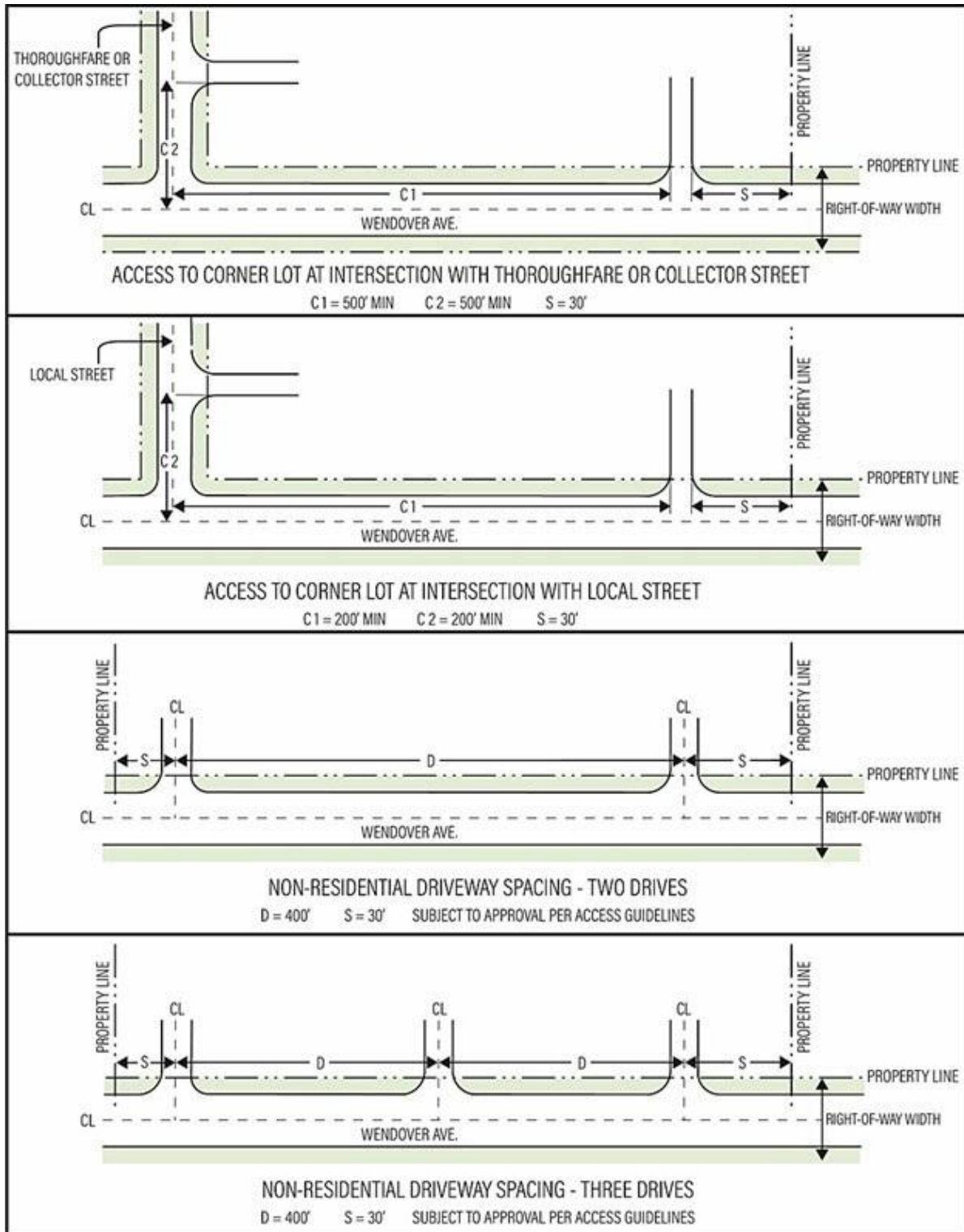
LOCATION AND SPACING OF DRIVEWAY ACCESS
